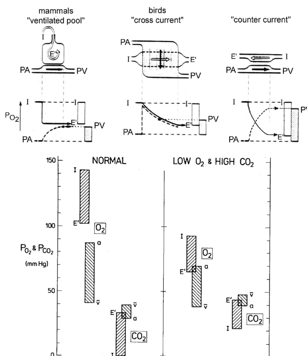
Figure 6. Top , models for gas exchange. In cross- and countercurrent models the O 2 tension can be greater in blood leaving the lung (pulmonary venous, PV) than it is in the expired gases of the lung (E'). I = inspired air, PA = pulmonary arterial blood. After Meyer et al. (1981). Bottom , tension of oxygen and carbon dioxide in the blood and lung gas in the domestic fowl, from Scheid and Piiper (1987). I, E', a, and v refer to inspired, end-expired, arterial, and mixed venous partial pressure of oxygen (P O 2 ) and carbon dioxide (P CO 2 ) values. Note the reversal in the gradient for O 2 when the animals breathed a gas mixture low in O 2 and high in CO 2 (fraction of inspired gas: O 2 = 0.12, CO 2 = 5.0).
