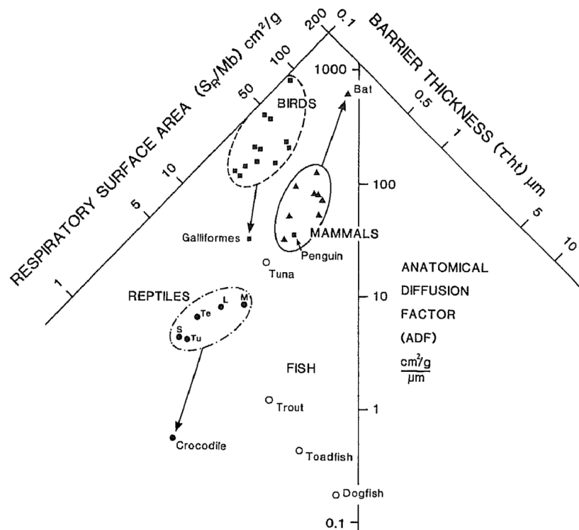
Figure 3. Triple logarithmic plot of mass-specific harmonic mean thickness of the blood gas barrier, the respiratory surface area, and the anatomical diffusion factor (ADF). L , Lacerta spp.; M , Varanus exanthematicus ; S , Pituophis melanoleucus ; Te , Tupinambis nigropunctatus ; Tu , Trachemys scripta elegans . Graph is modified from Perry (1990b).
